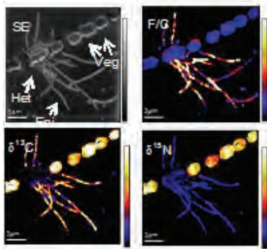
Figure. NanoSIMS images of a chain of 8 cells from the filamentous cyanobacterium Anabaena sp. SSM-00 with cells of the \alpha -Proteobacterium epibiont Rhizobium sp. WH2K attached to a heterocyst. Images were taken after 24 h of incubation with \text{H}^{13}\text{CO}_3^- and ^{15}\text{N}_2 . SE: Secondary electron image showing the location of all cells. F/C: Fluorine is enriched in the epibiont relative to Anabaena after in situ hybridization with an \alpha -Proteobacteria specific probe (scale, 0 – 0.2). \delta^{13}\text{C} : ^{13}\text{C} enrichment image showing the relative uptake of newly fixed carbon (scale, 0 – 300 parts per thousand). \delta^{15}\text{N} : ^{15}\text{N} enrichment image showing the relative uptake of newly fixed nitrogen (scale 0 – 15,000 parts per thousand). The color bars indicate the relative enrichment of the isotope in the image. Het, heterocyst; Veg, vegetative cells; Epi, epibiont.
