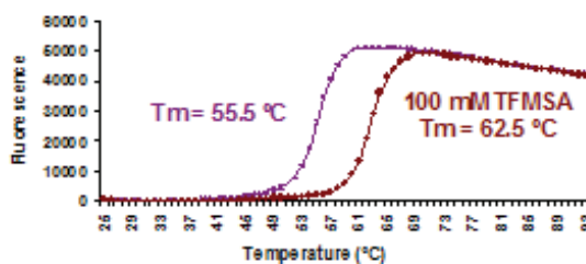
Fig. 1b. Thermal shift assay using 10 μM CAI and 5X SYPRO orange dye with and without ligand (100mM TFMSA)
