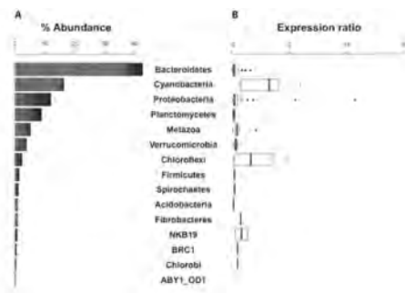
Figure 2. (A) More than 63 phyla across all domains of life were present in the upper 2 mm strata as determined by rDNA sequencing (15 most abundant phyla shown). (B) OTUs belonging to Cyanobacteria and Chloroflexi had relatively higher rRNA:rDNA ratios (expression ratios), suggesting that organisms in these phyla are more active relative to organisms in other phyla present in the mats.
