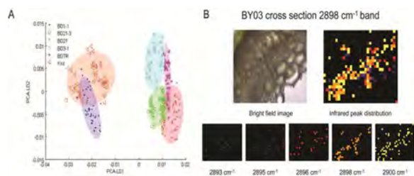
Figure 2. Chemical analysis of Brachypodium samples using mid-IR. (A). The PCA-LDA score plot of samples from 6 Brachypodium lines. 45 spectra are collected from each line. Spectra data are collected from 600 \text{cm}^{-1} to 4000 \text{cm}^{-1} . The spectra in the region between 800 \text{cm}^{-1} and 1200 \text{cm}^{-1} are used as input for PCA-LDA analysis. The “Bd1-1” and “Koz-3” samples are clearly separated from the other 4 types of samples. (B). The distribution and shift of the 2898 \text{cm}^{-1} band in the cross section of a Brachypodium sample thin slice. Each peak position is represented by a different color.
