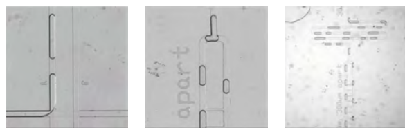
Figure 2. Photos showing droplet generation, mixing, and queuing.
