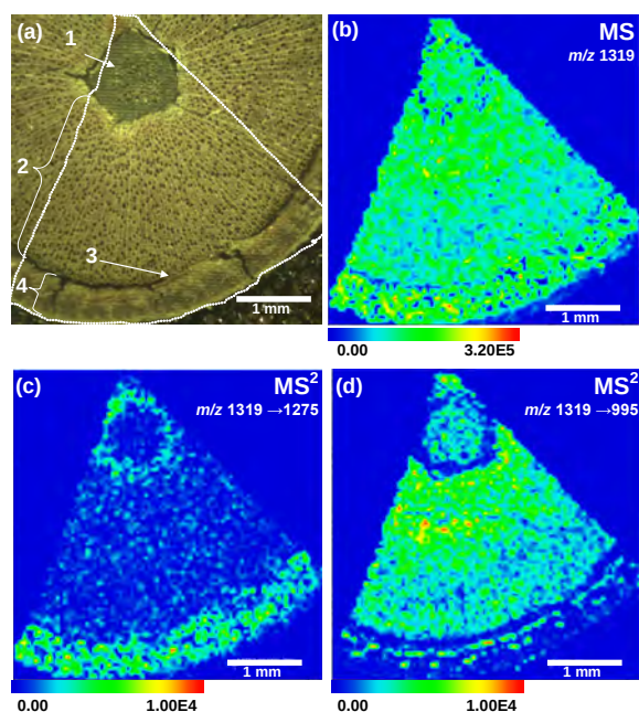
Figure 1. a) optical image, b) MS of m/z 1319, c) MS 2 of m/z 1319-1275, d) MS 2 of m/z 1319 to 995
