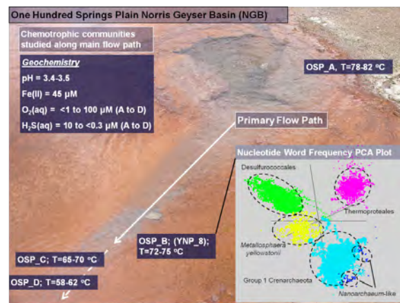
Figure 1. Site photograph of Fe-oxide depositing geothermal spring (One Hundred Spring Plain, OSP) located in Norris Geyser Basin (YNP). Reduced geothermal waters emerge with little to no detectable dissolved oxygen and significant levels of ferrous Fe (~50 µM). The oxidation of Fe(II) to produce amorphous Fe(III)-hydroxide is catalyzed by microbial populations such as Metallosphaera yellowstonensis . Inset at right indicates predominant microbial populations present at OSP_B (~72-75 °C) identified using nucleotide word frequency plots of assembled metagenome sequence.
