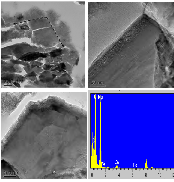
Figure 2. Crystallites from upper layer of the Hot Lake mat sampled just above the green cyanobacterial layer. The crystallites are magnesite ( \text{MgCO}_3 ) as determined by selected area electron diffraction (SAED) with amorphous coatings of similar elemental composition as determined by energy dispersive X-ray spectroscopy (EDS).
