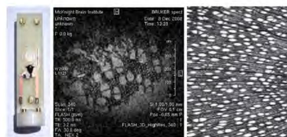
Figure 2. Using the new rf microcoils (left) this figure shows an MR microimage (8 microns, 4hrs 33 min) of a wood chip sample (middle) with example optical histology 5X objective.
