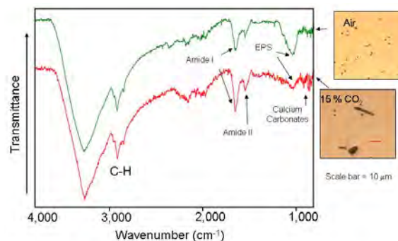
Figure 2. SR-FTIR spectra of calcification in the cyanobacterium Synechococcus 8802.
